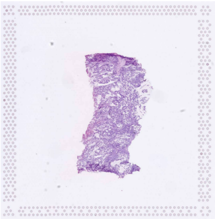
Original H&E
