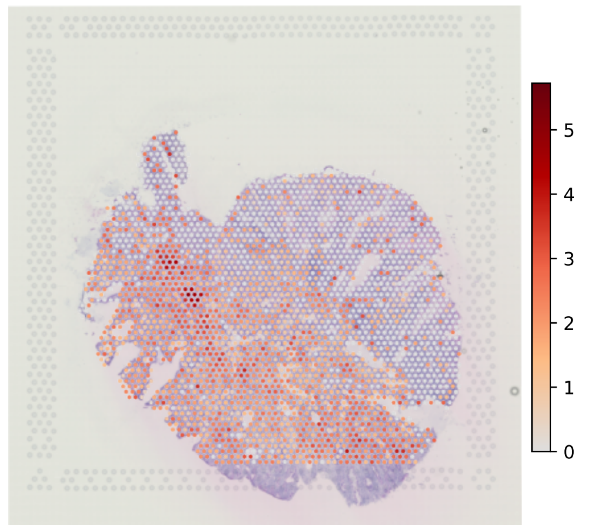
COL1A1 | log1p CP10K
