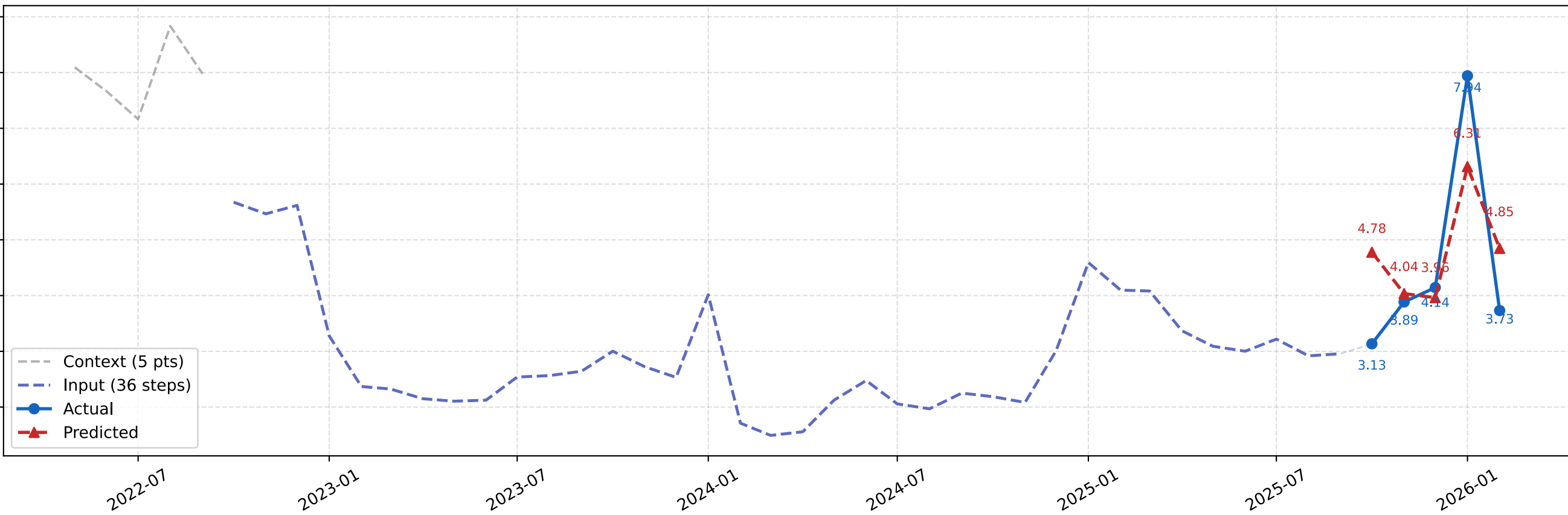
Forecast | natural_gas
