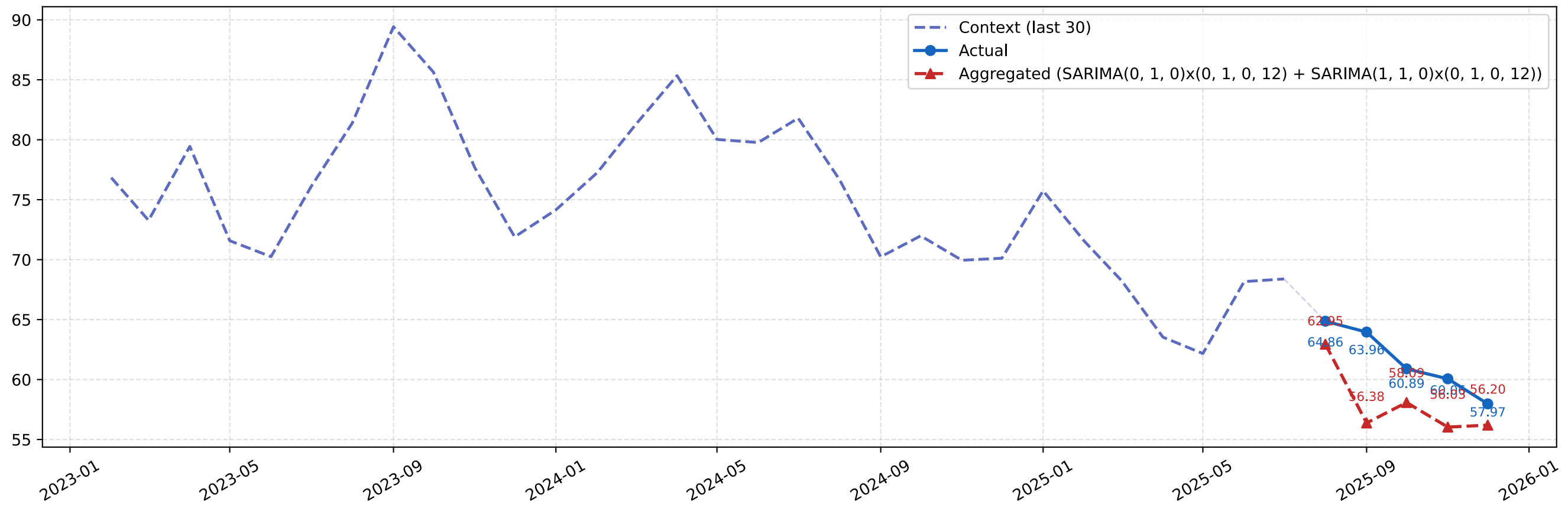
Forecast | wti_crude_oil Best 2 Aggregated
