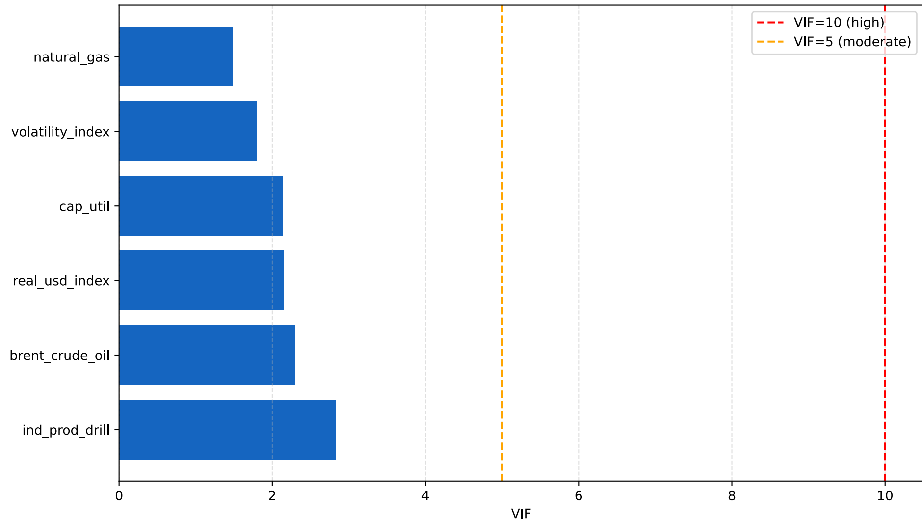
Variance Inflation Factor (VIF)
