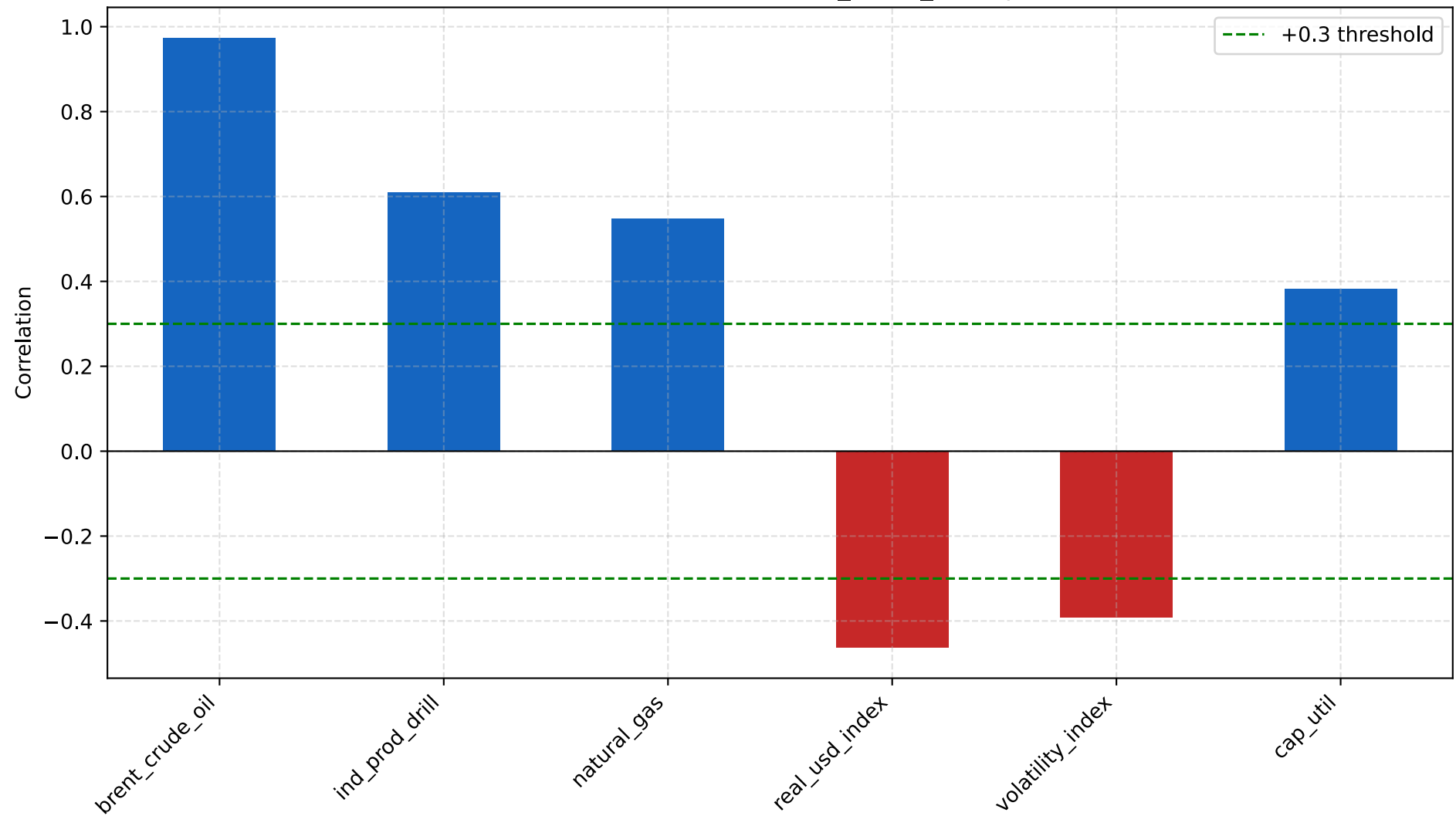
Pearson Correlation with wti_crude_oil (Top 20)
