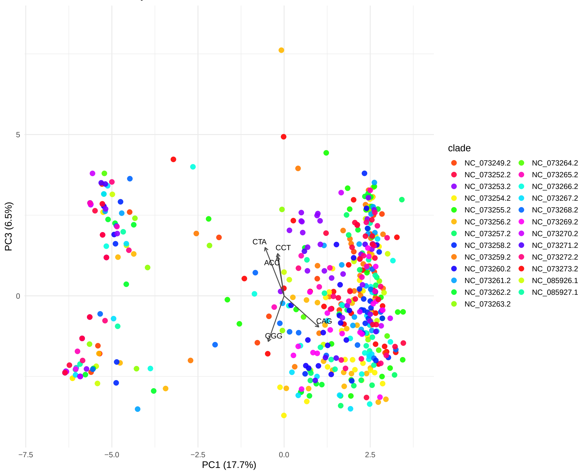
PC1 vs PC3 Colored by clade
