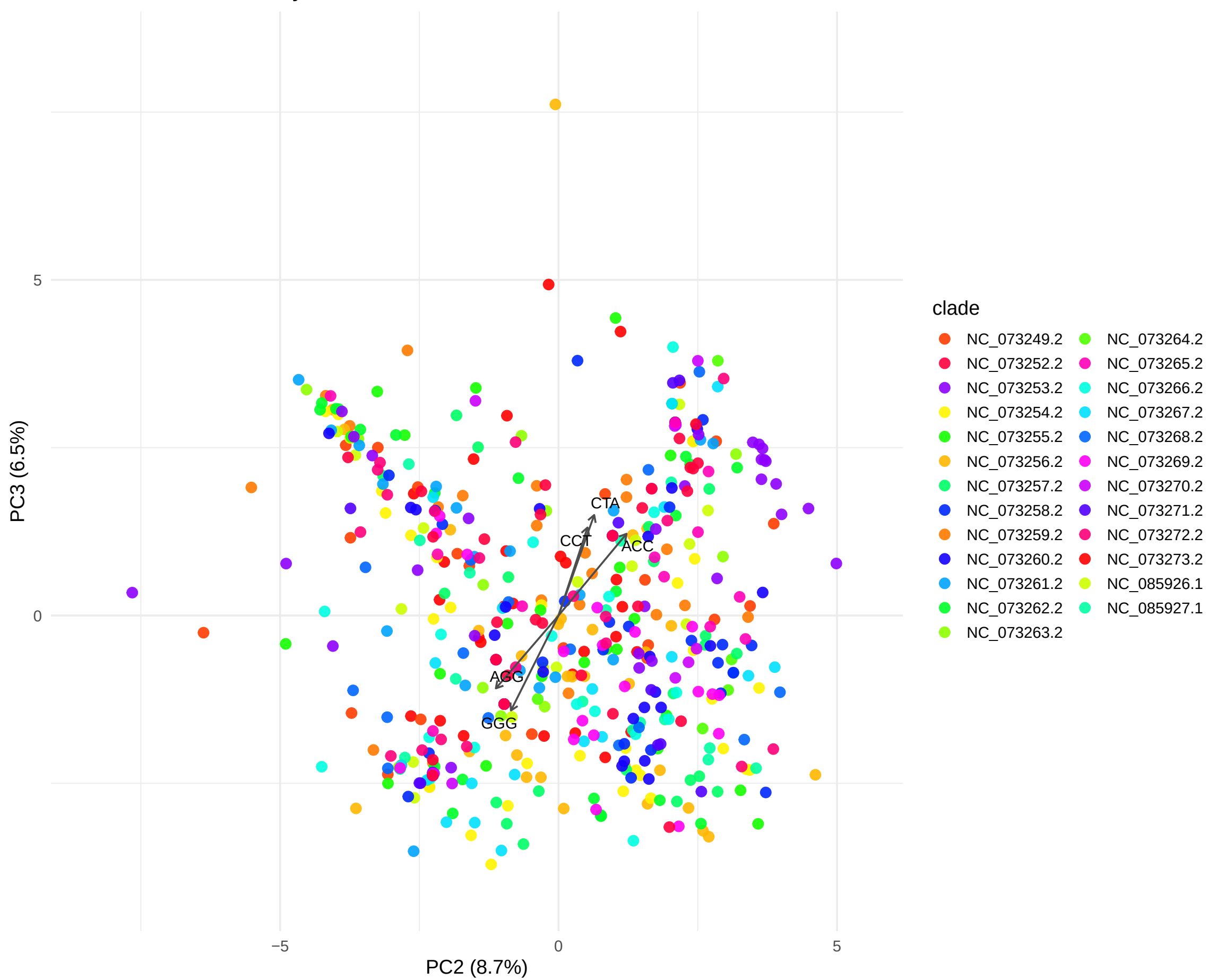
PC2 vs PC3 Colored by clade
