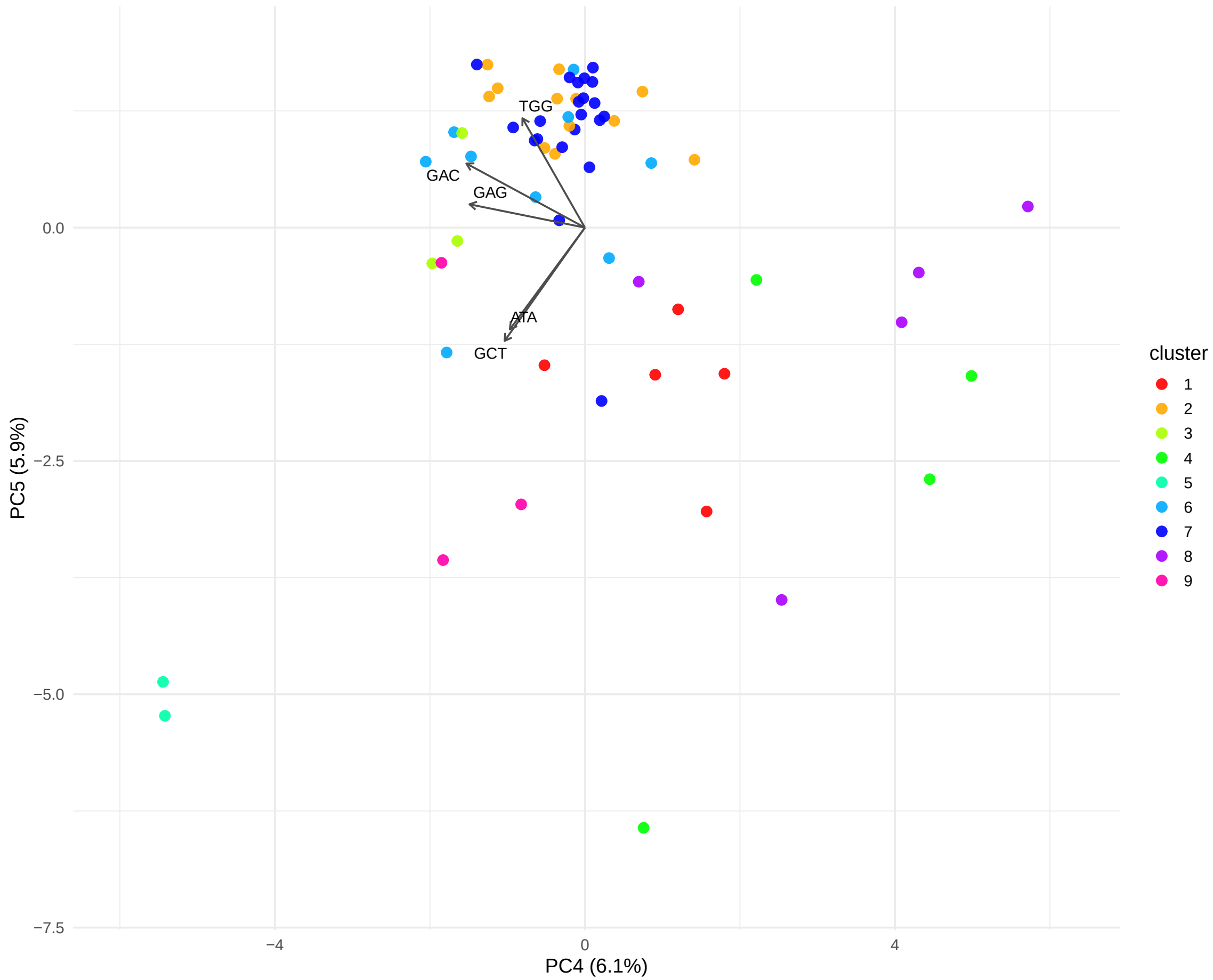
PC4 vs PC5 Colored by cluster
