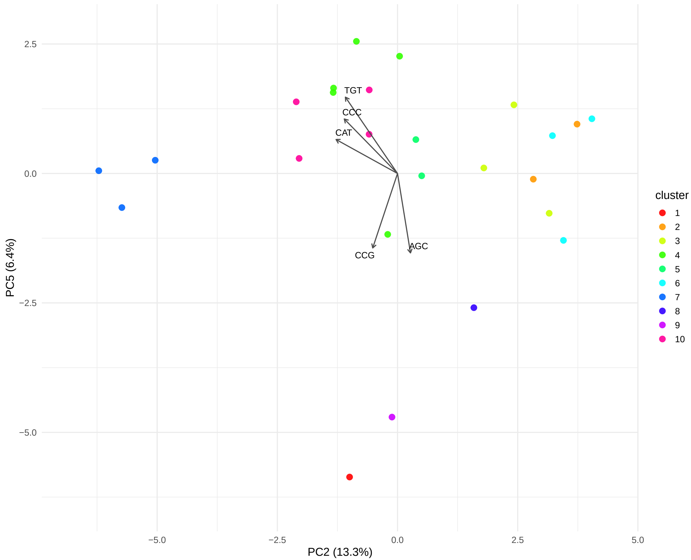
PC2 vs PC5 Colored by cluster
