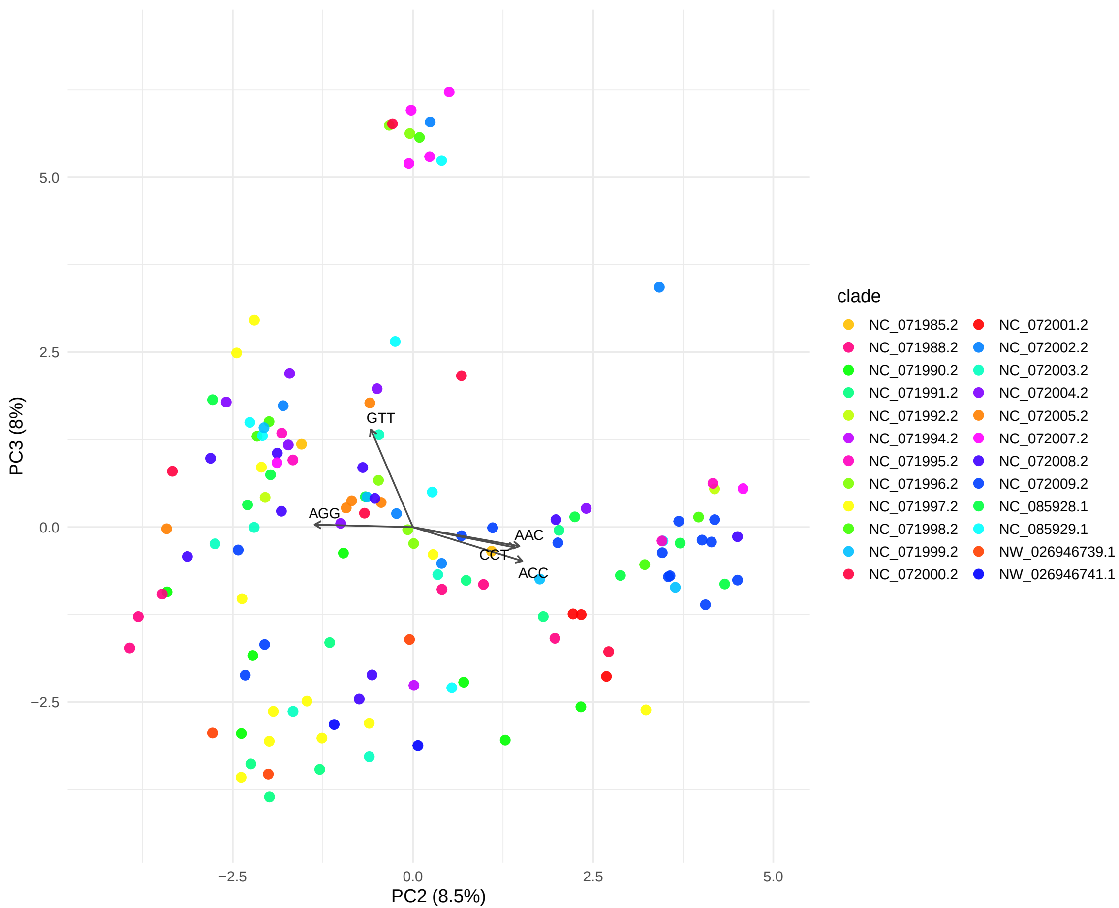
PC2 vs PC3 Colored by clad
