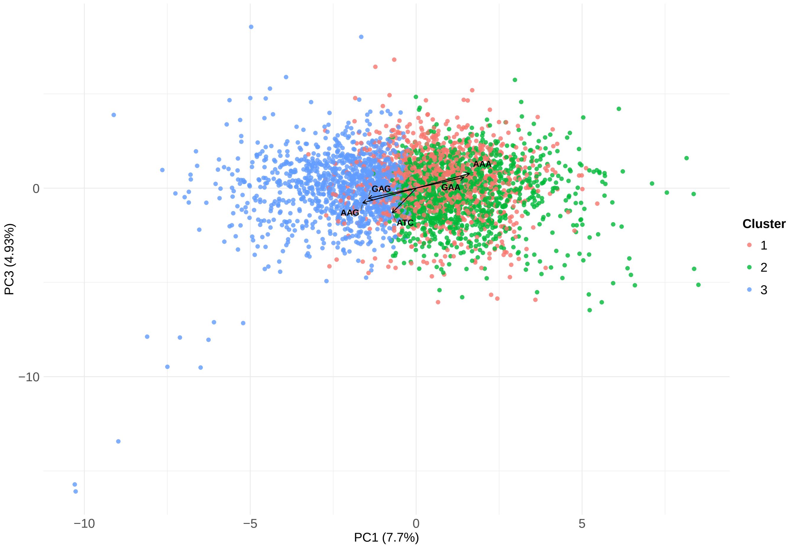
borangutan – genes – PC1 vs PC3
