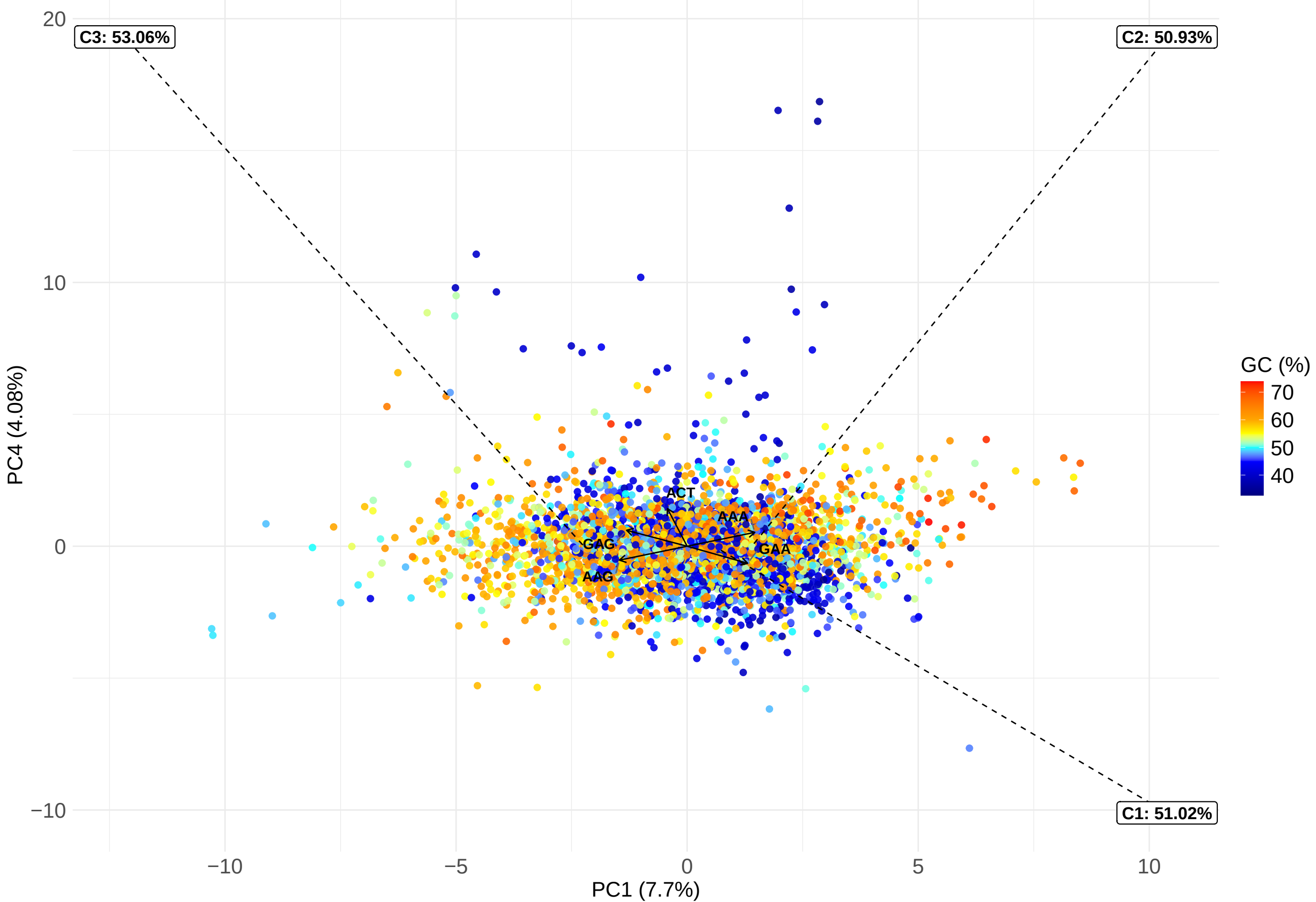
borangutan – genes – PC1 vs PC4
