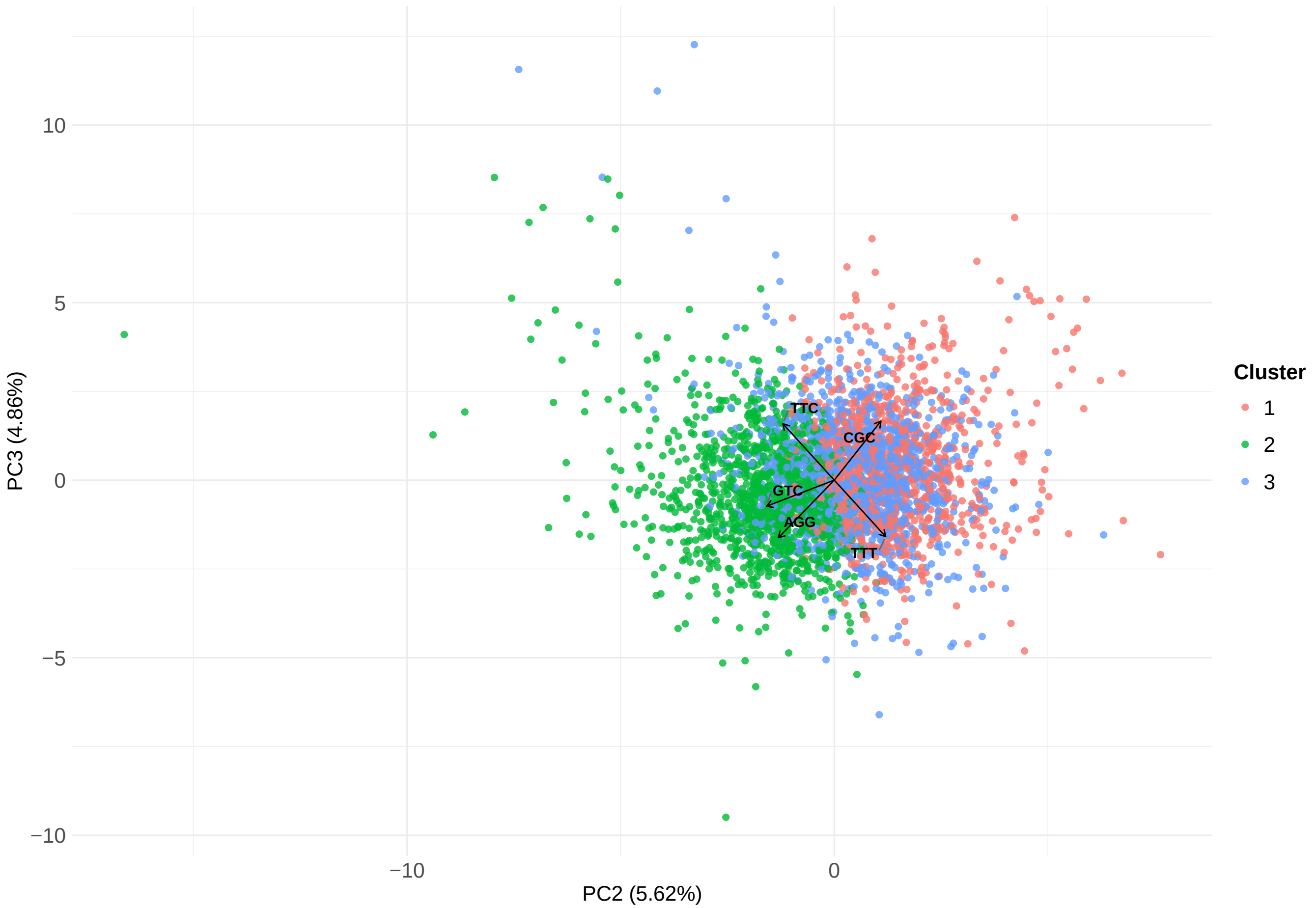
chimpanzee – genes – PC2 vs PC3
