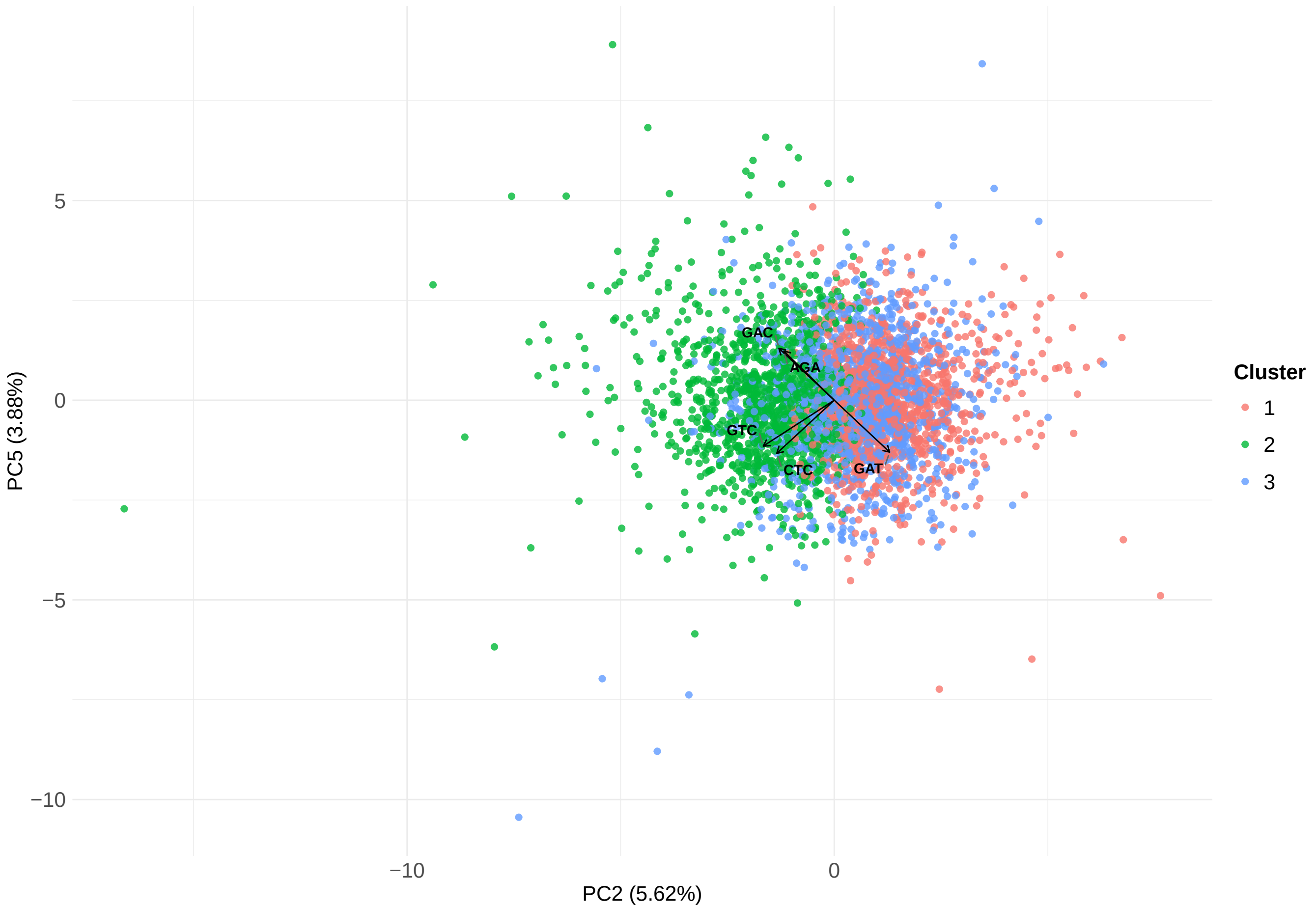
chimpanzee – genes – PC2 vs PC5
