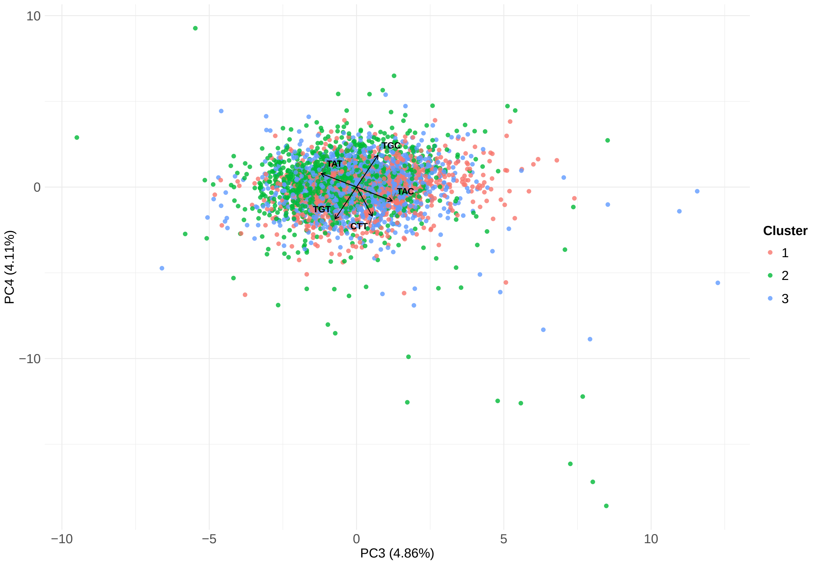
chimpanzee – genes – PC3 vs PC4
