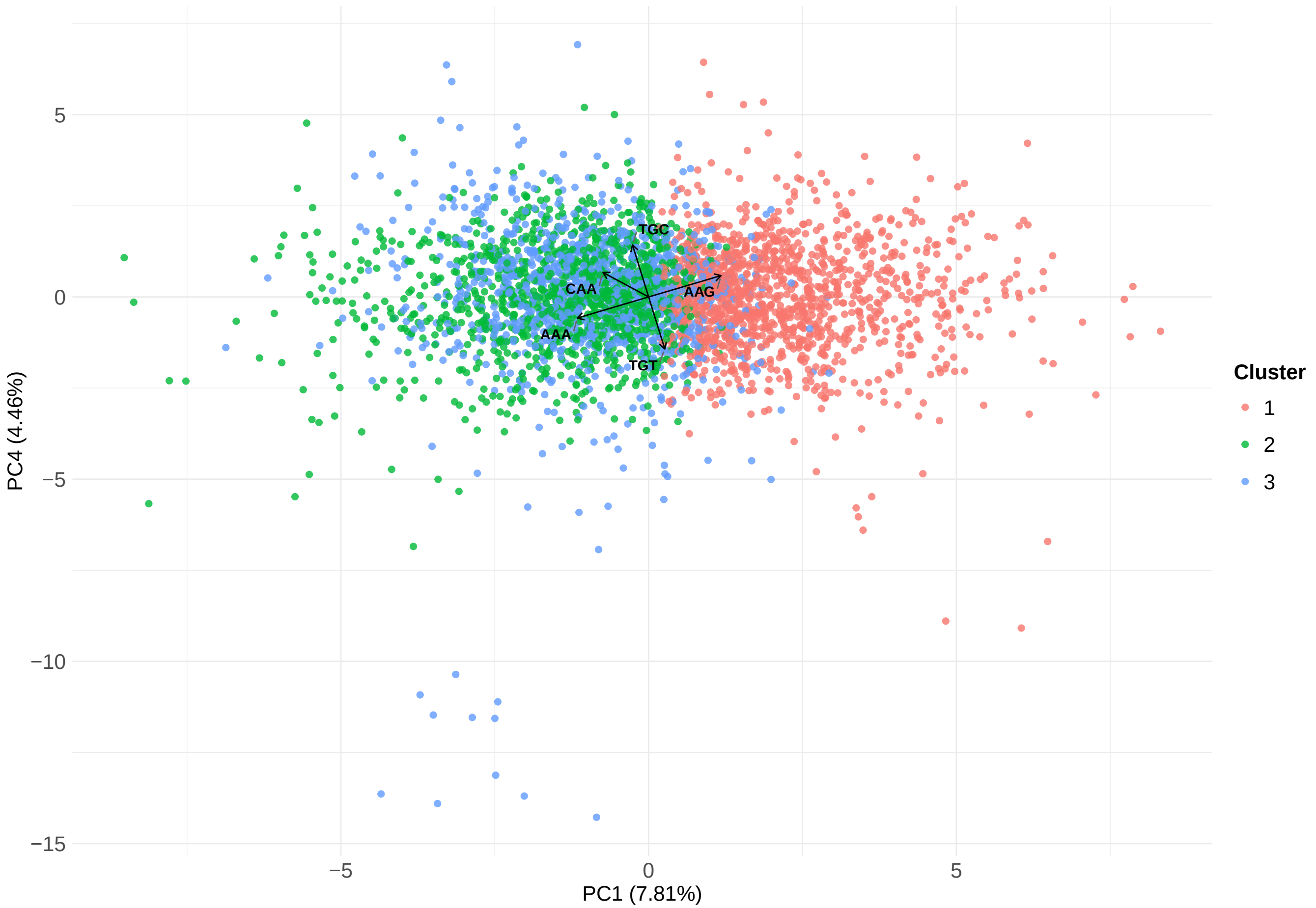
gibbon – genes – PC1 vs PC4
