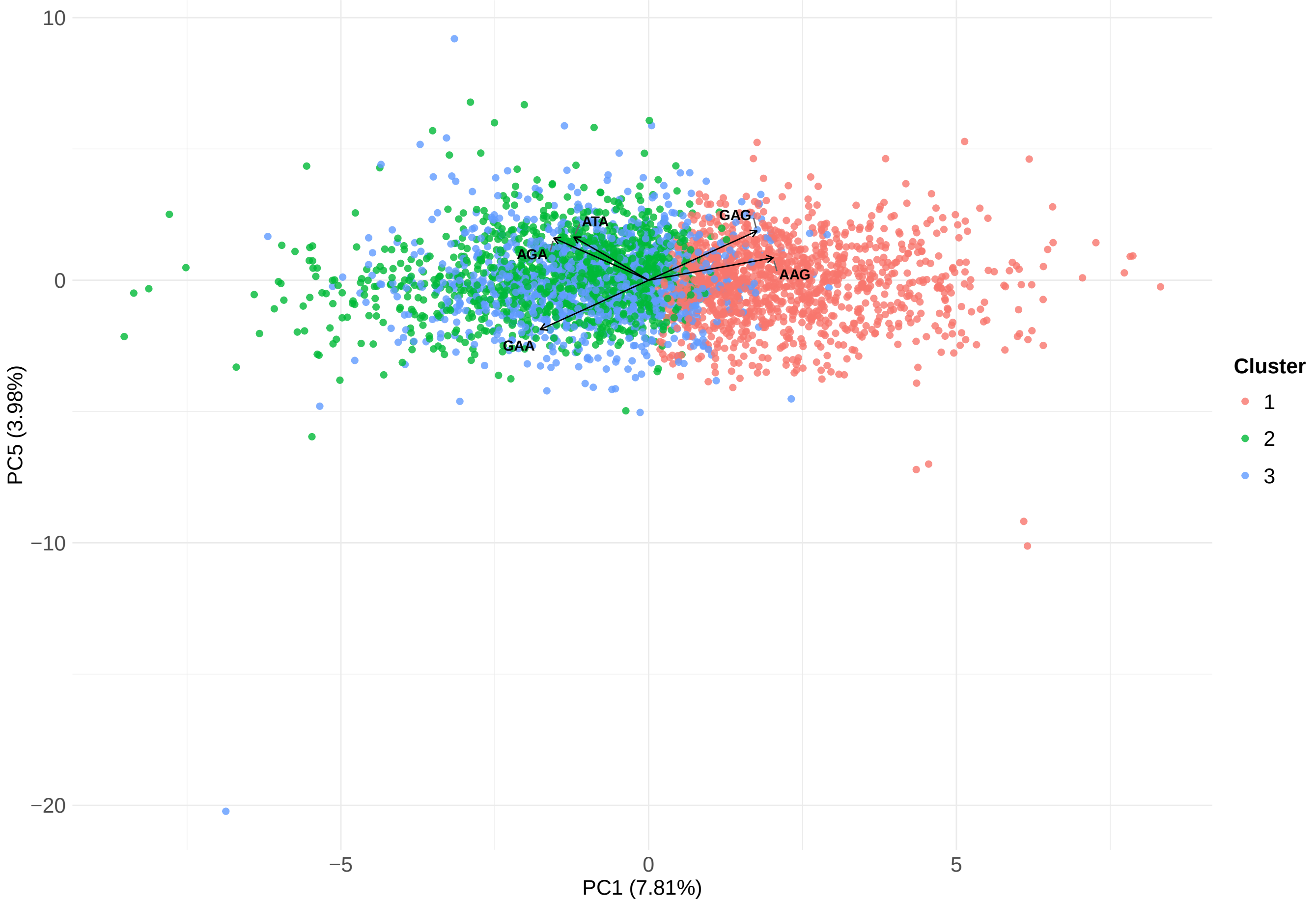
gibbon – genes – PC1 vs PC5
