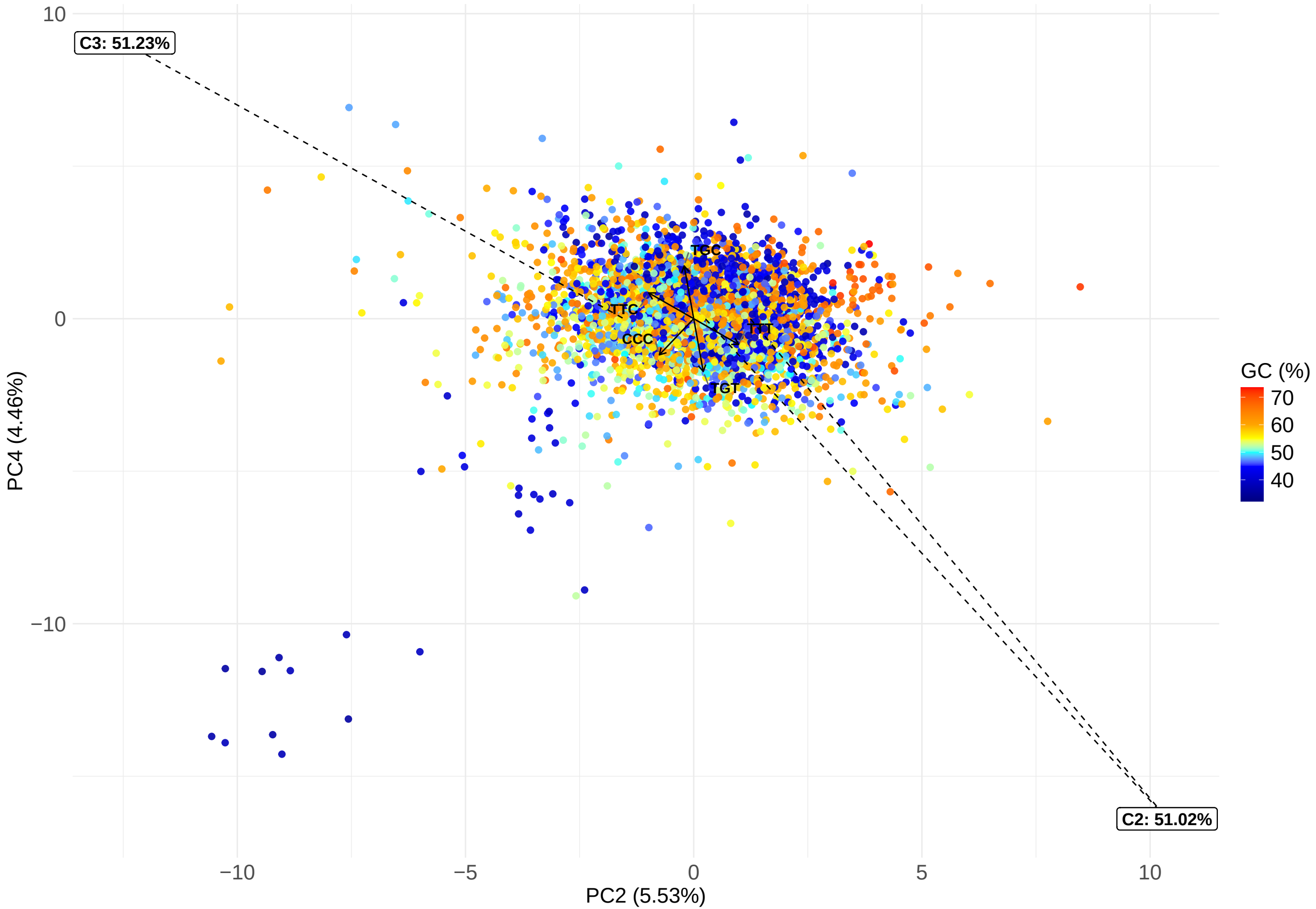
gibbon – genes – PC2 vs PC4
