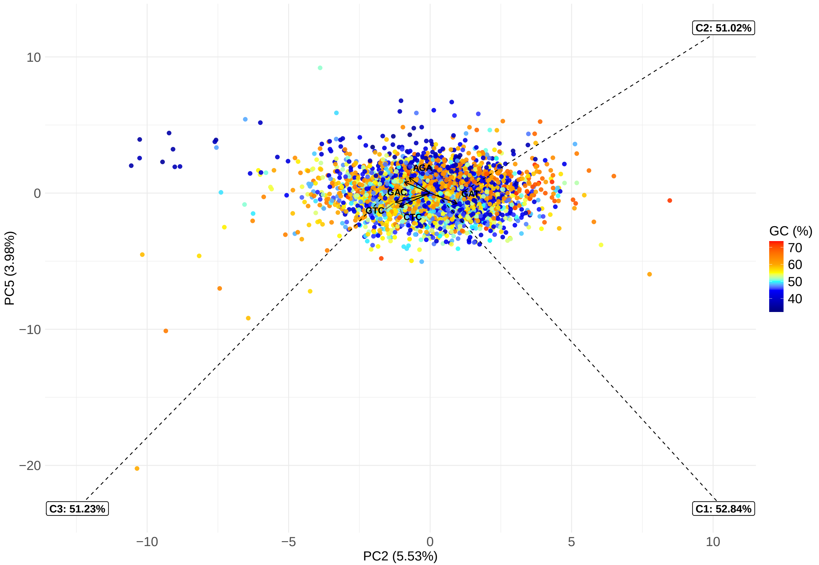
gibbon – genes – PC2 vs PC5
