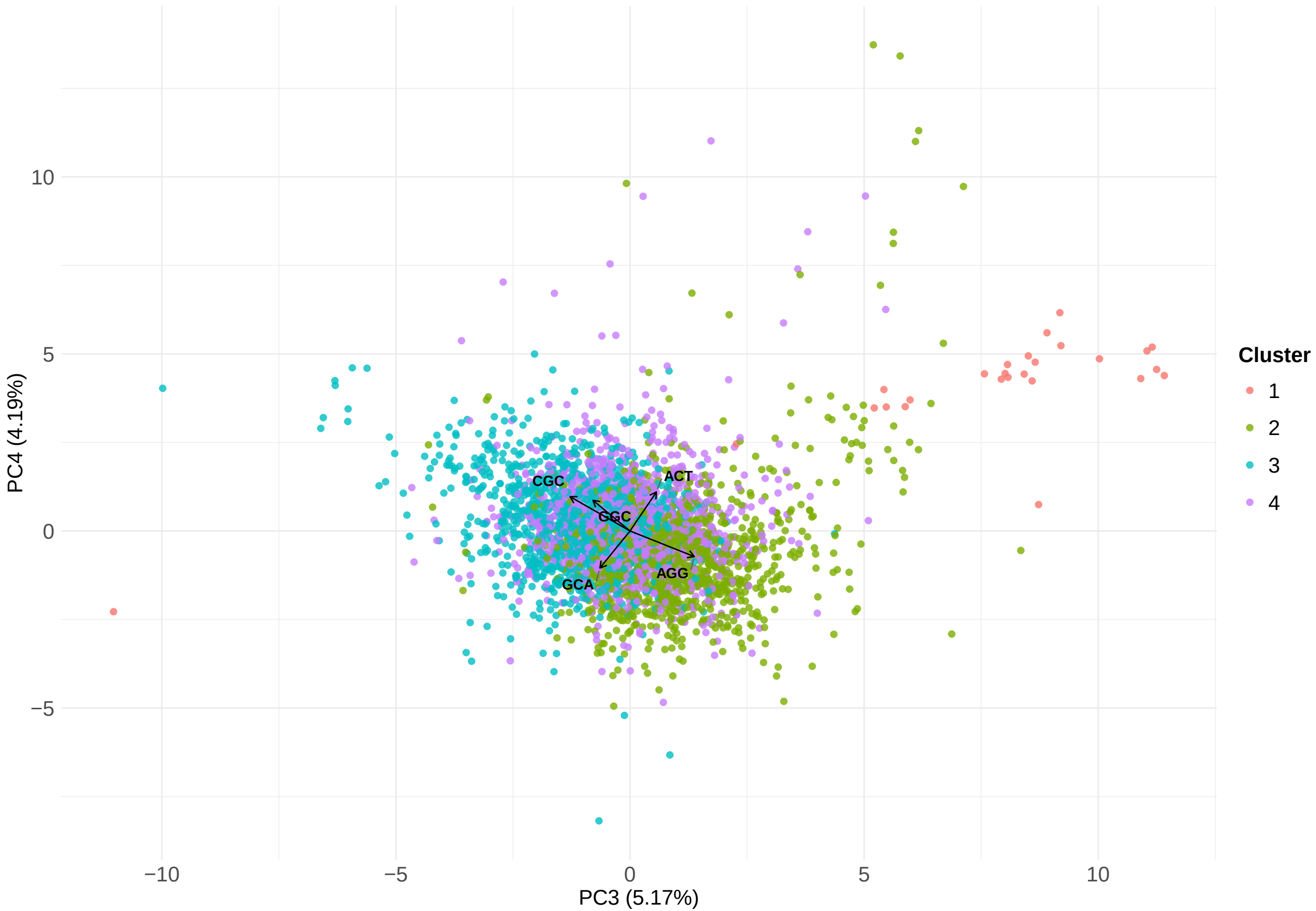
gorilla – genes – PC3 vs PC4
