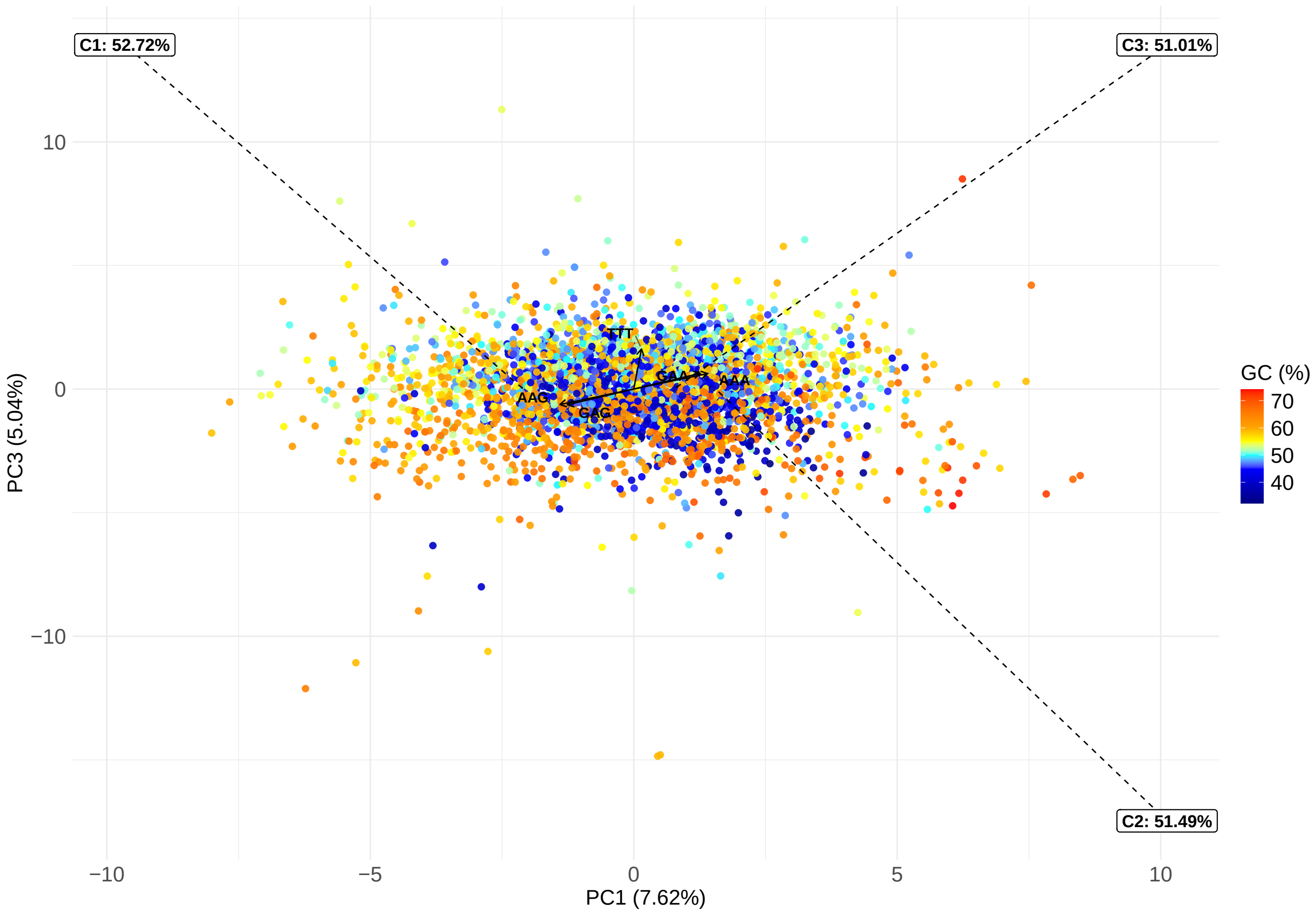
human – genes – PC1 vs PC3
