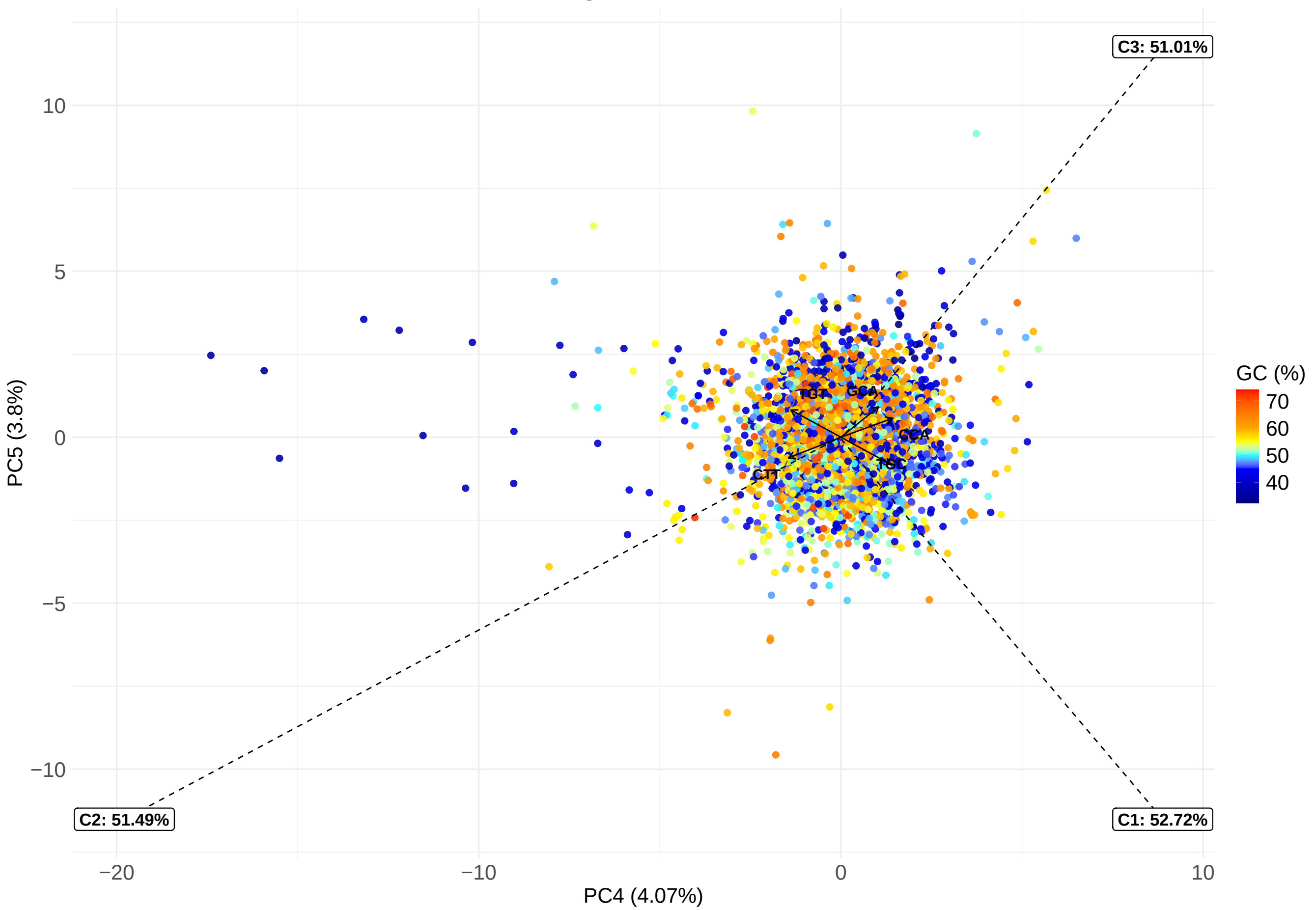
human – genes – PC4 vs PC5
