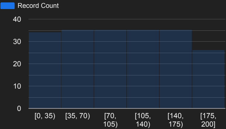
Distribution of rank
