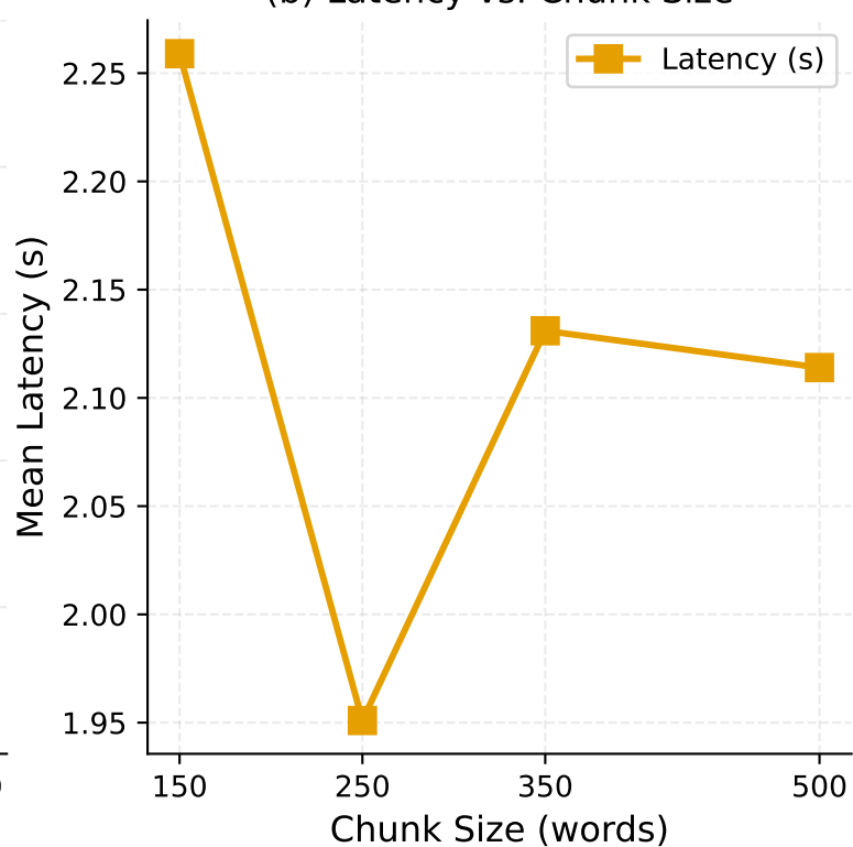
(b) Latency vs. Chunk Size
