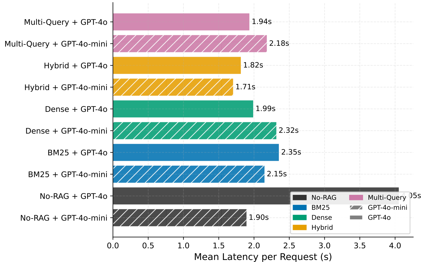
Response Latency by Pipeline and Model
