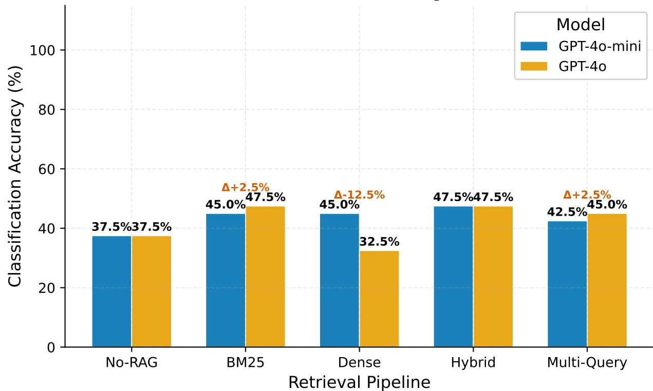
GPT-4o vs GPT-4o-mini Accuracy per Pipeline ( \Delta = GPT-4o advantage)
