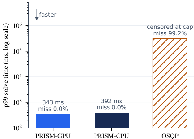
B. p99 timing and deadline misses
