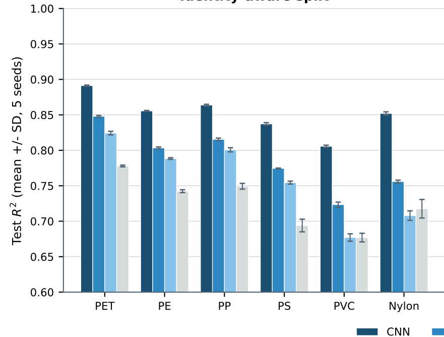
Identity-aware split
