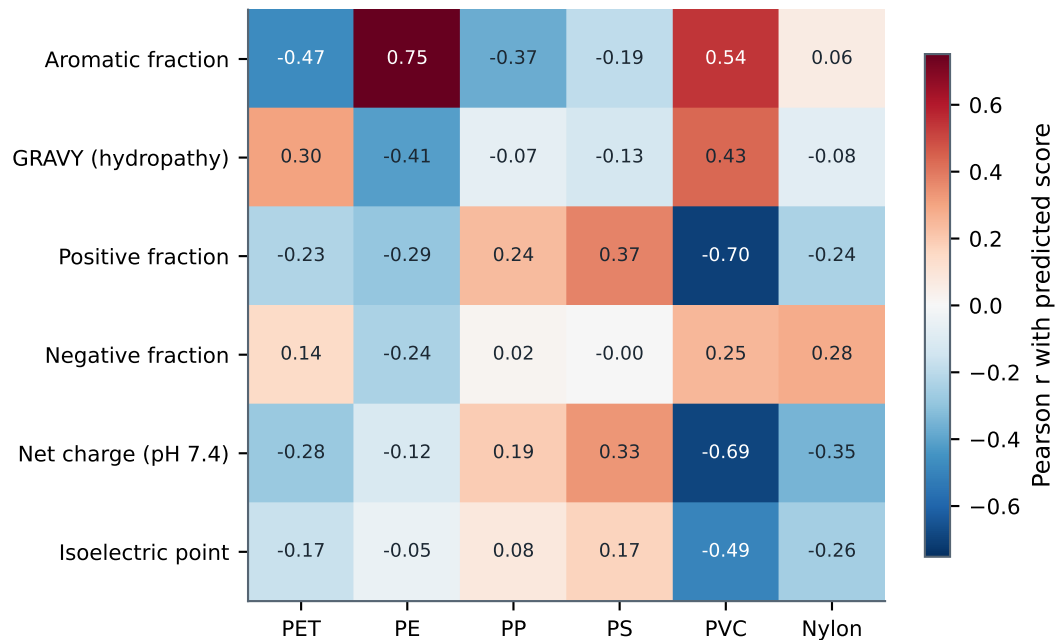
(a) Property-affinity relationships
