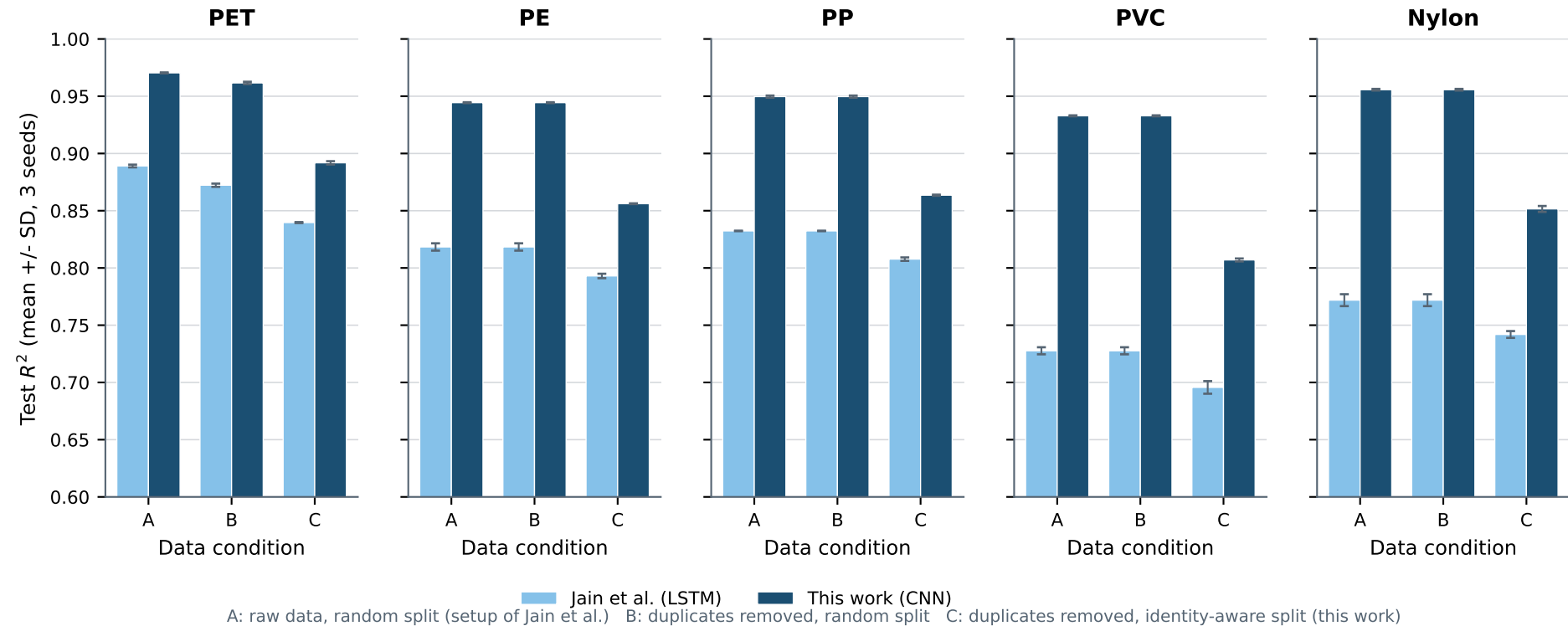
Benchmark against Jain et al. (2025) under three data conditions
