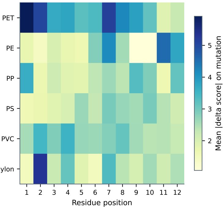
(a) Positional sensitivity of the model
