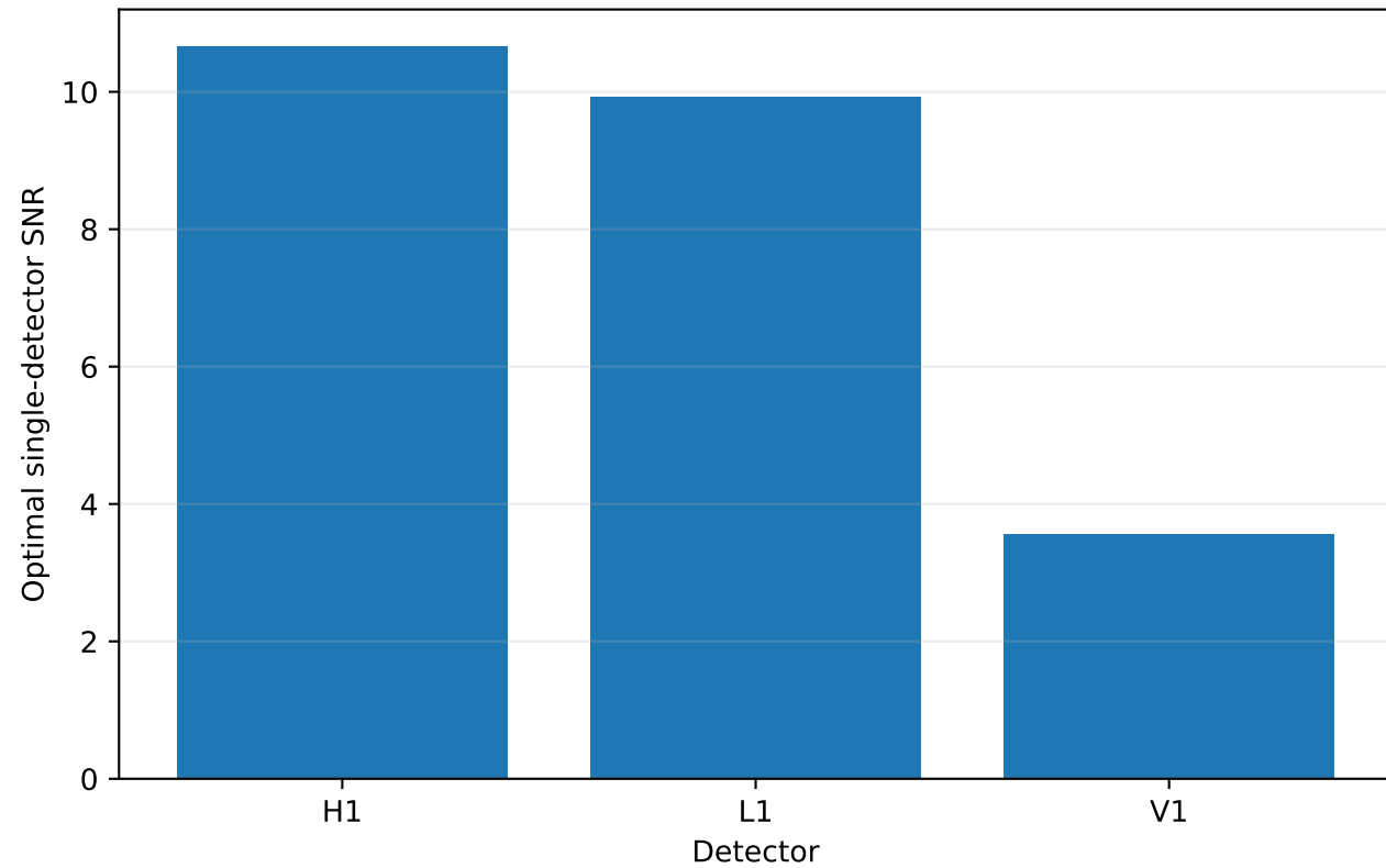
Injected memory signal across synthetic detector network
