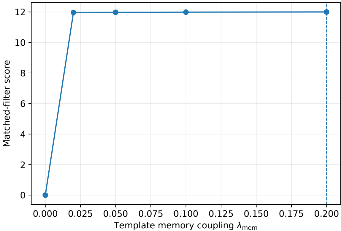
Template recovery in synthetic colored noise
