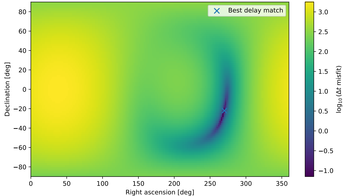
Toy sky-delay misfit map
