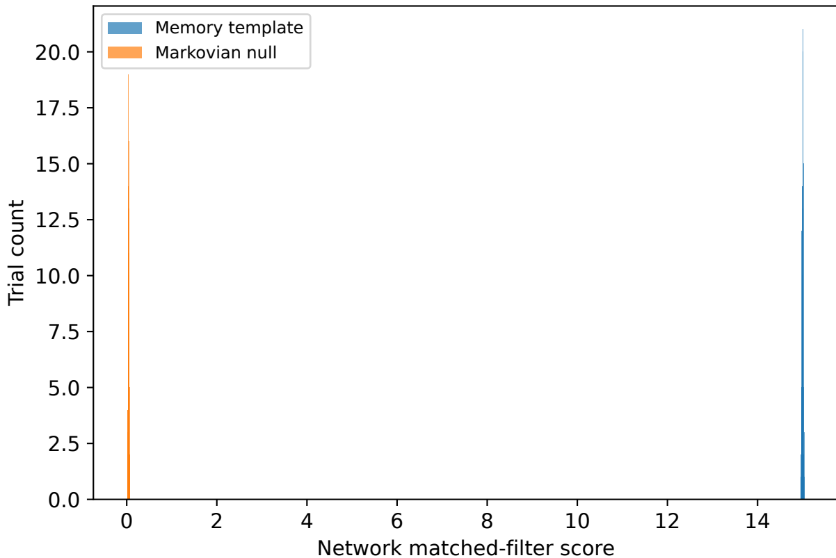
Network recovery: memory template versus null
