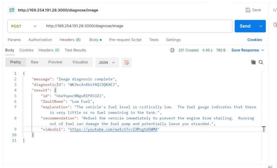
Fig 21: Test response in postman
