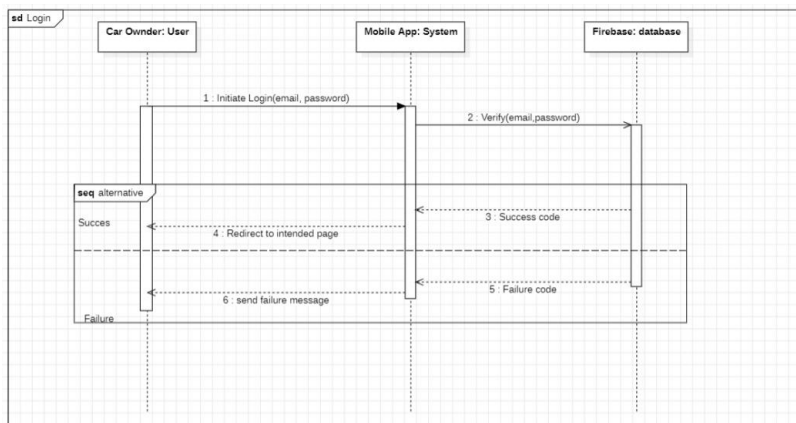
Fig4 : sequence diagram Login process
