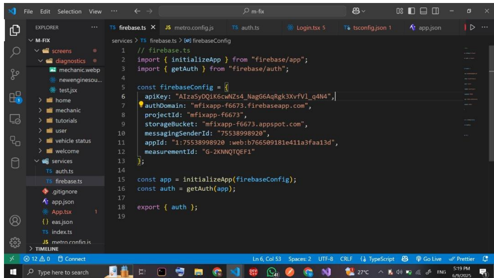
Fig 17: Firebase configuration for authentication
