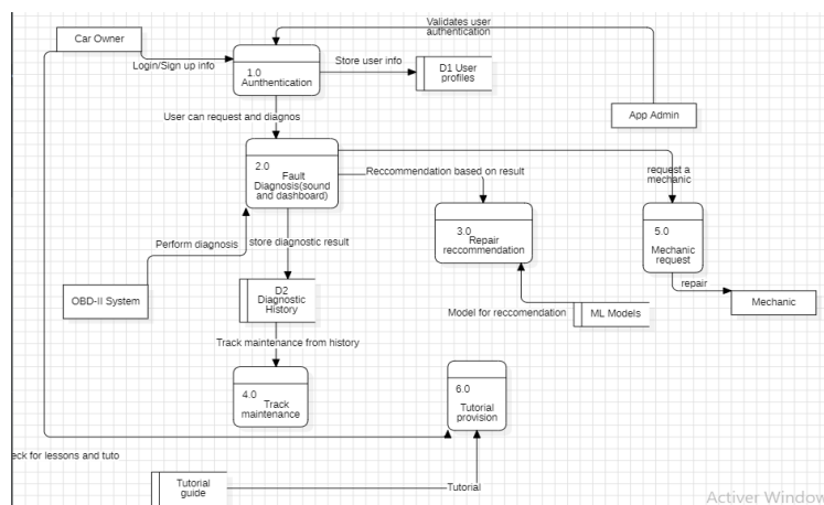
Fig9: Dataflow diagram
