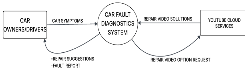
fig10: context diagram
