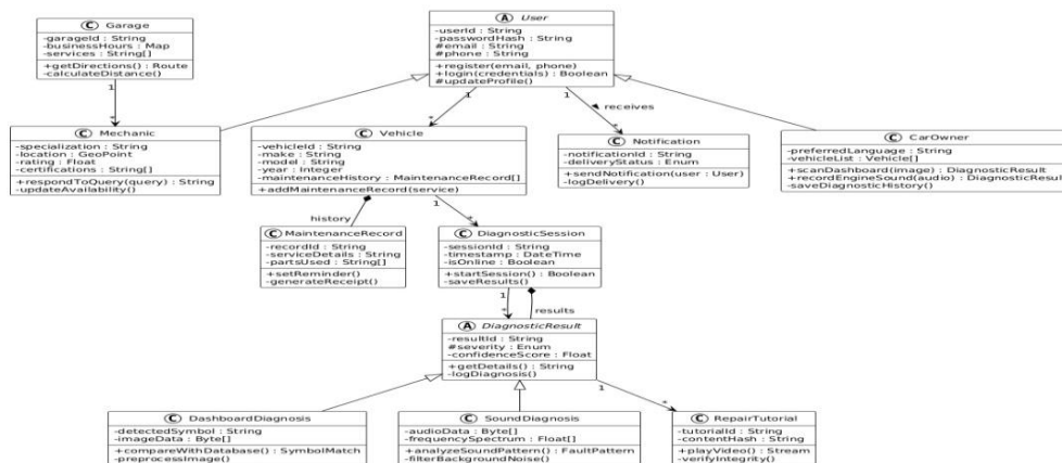
Fig11: Class Diagram
