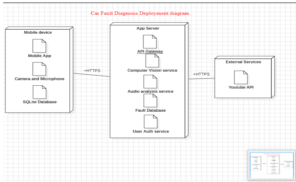
Fig12: deployment diagram
