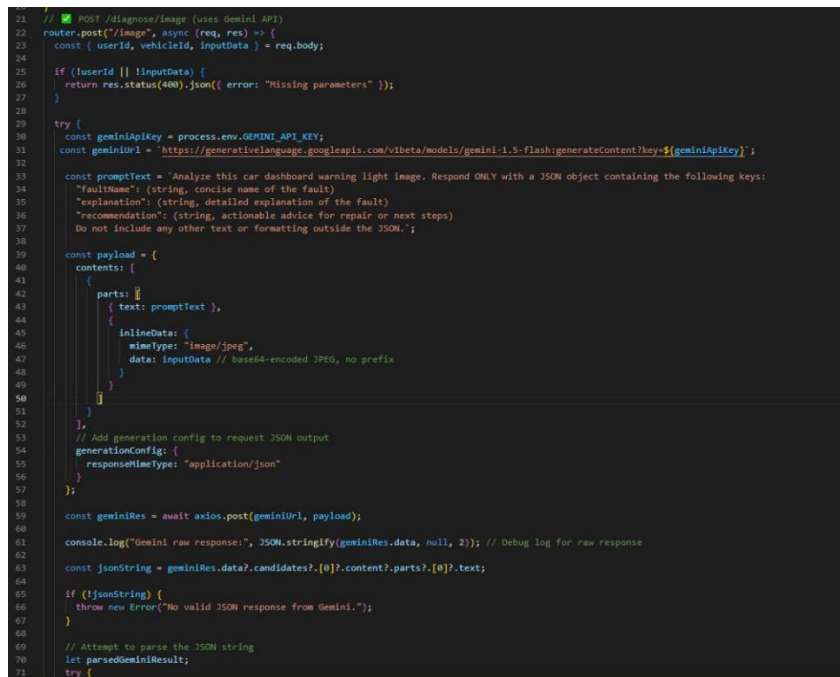
Fig18: Image diagnosis code
