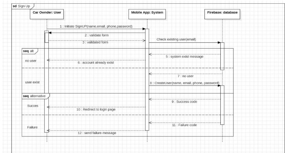
Fig5: sequence diagram, create account
