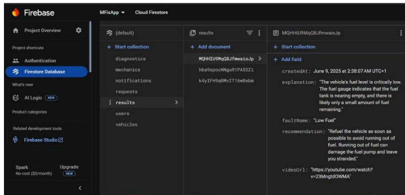
Fig 16 : Firebase Overview.
