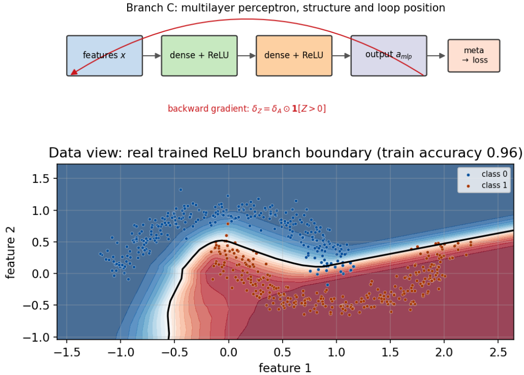
Figure 8: Branch C overview. The forward flow stacks two rectified layers before the meta layer, and the gradient is gated by \mathbf{1}[Z > 0] . The data view shows the nonlinear boundary the rectified layers can represent.
