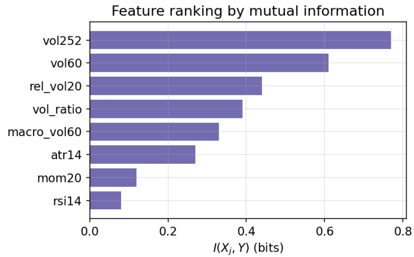
Figure 12: Features ranked by mutual information with the volatility label. The realized volatility over a long window carries the most bits, near 0.77.
