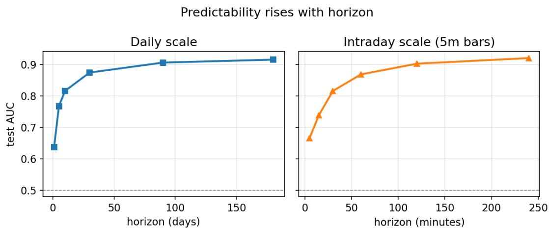
Figure 21: Test area under the curve by horizon. The daily scale climbs from about 0.64 at one day to about 0.92 at the long horizons, and the intraday scale climbs from about 0.67 at five minutes to about 0.92 at four hours.
