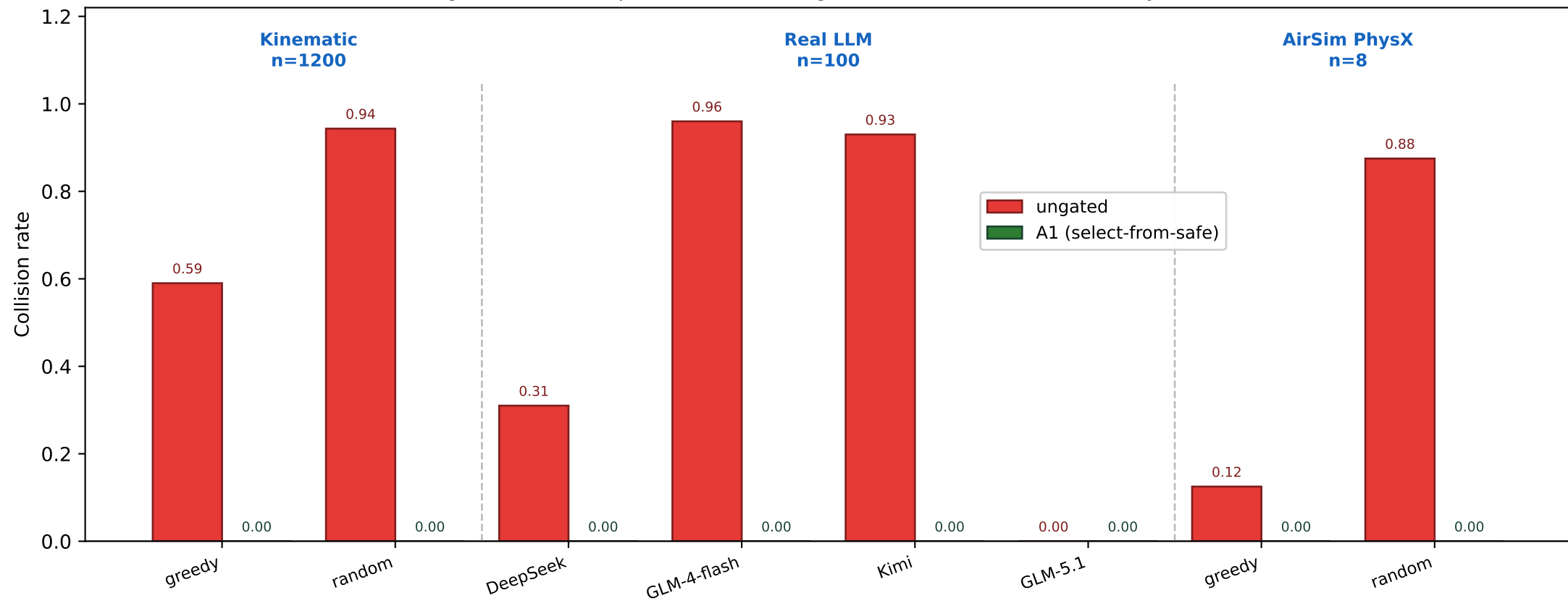
Fig 10 Closed-loop collision rate: ungated vs A1 across three fidelity levels
