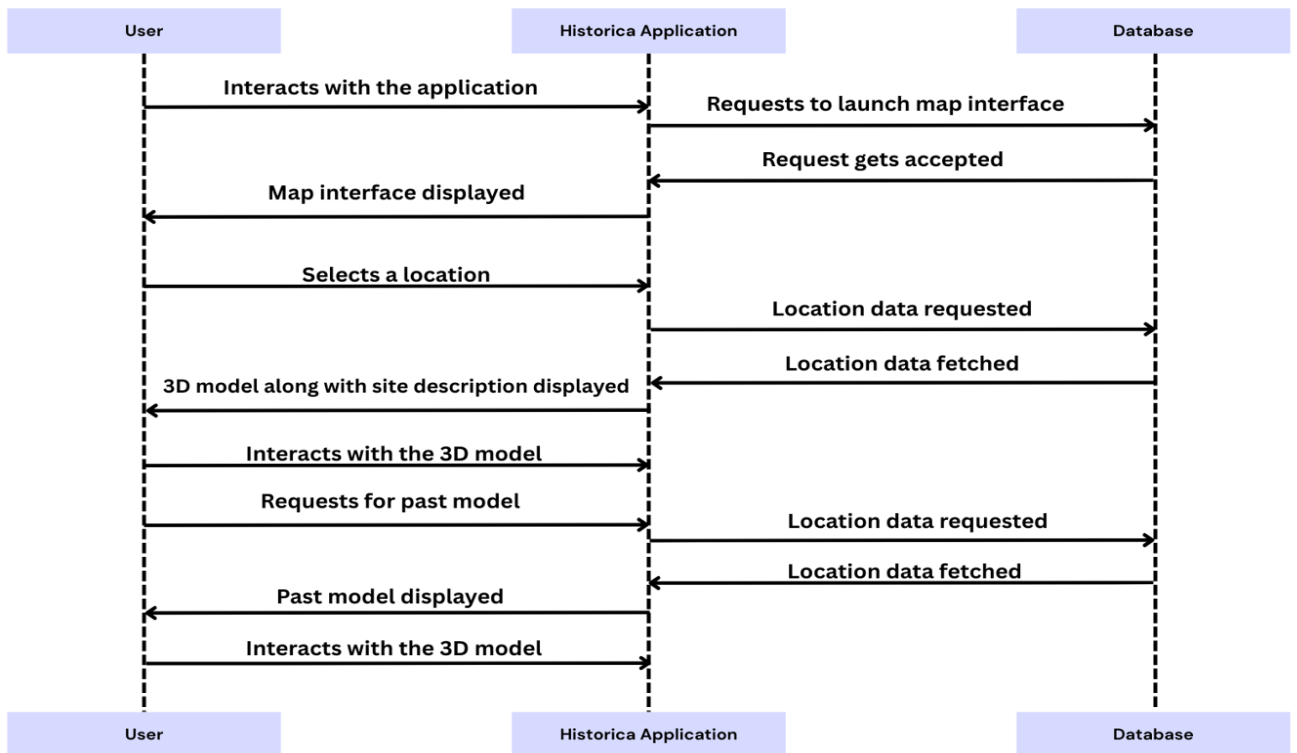
Fig. 3 Sequence Diagram
