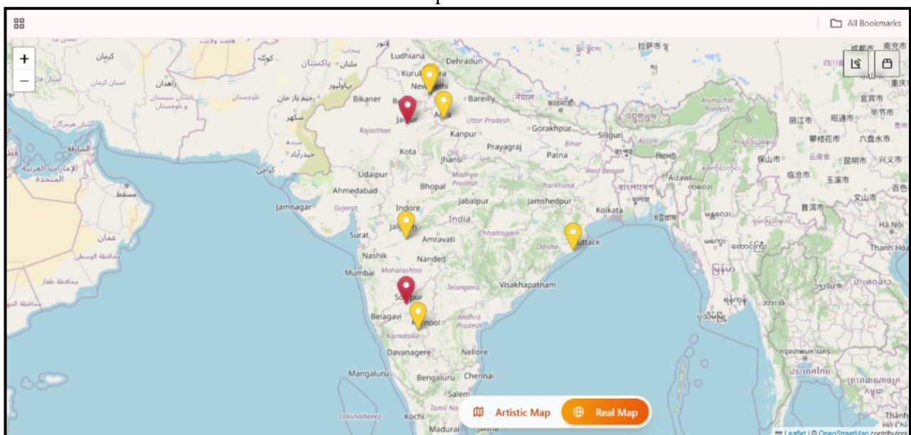
Fig.13 Map interface
