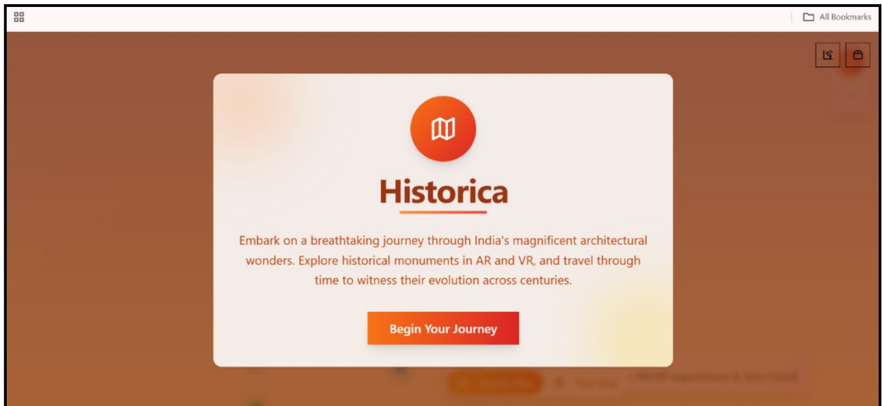
Fig. 6 Home page
