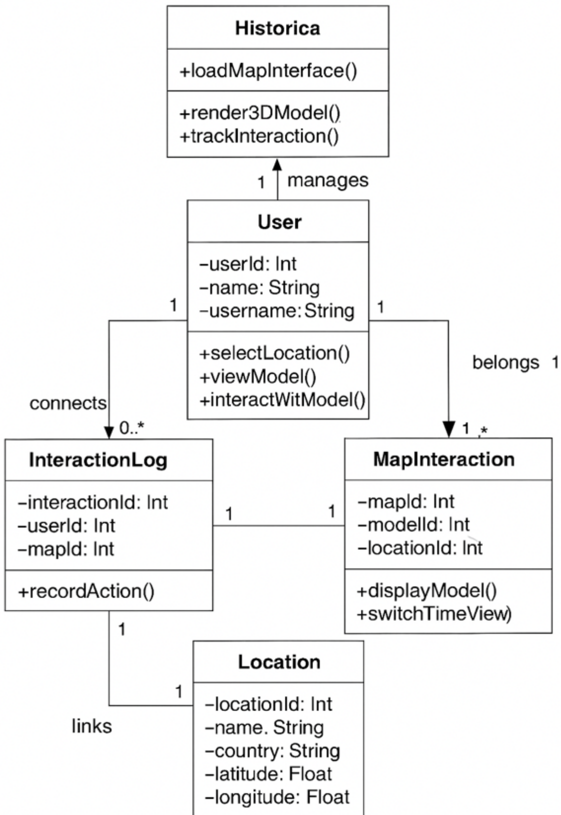
Fig. 4 Class Diagram
