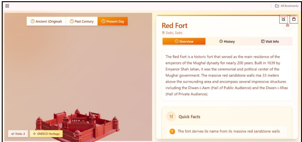
Fig.14 Model page
