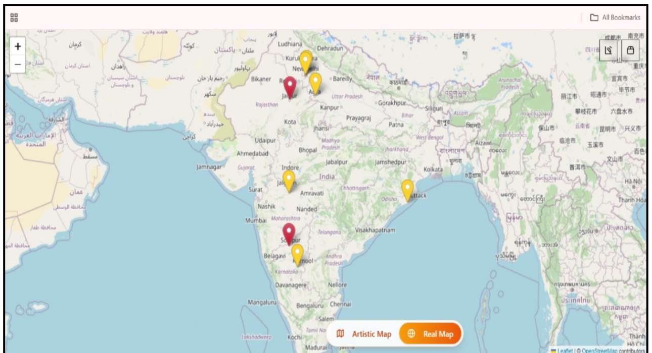
Fig. 7 Map interface
