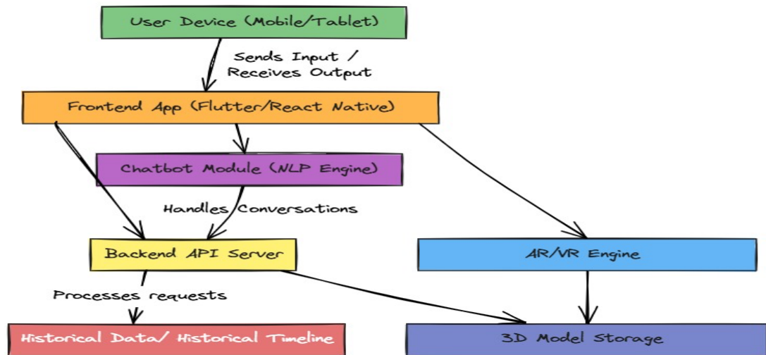
Fig. 2 Technical Architecture
