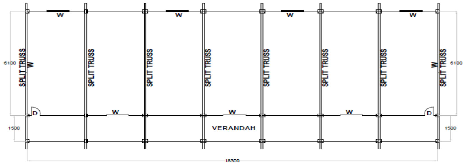
LAYOUT PLAN STORE SHELTER 18.30 X 6.10 MTR
