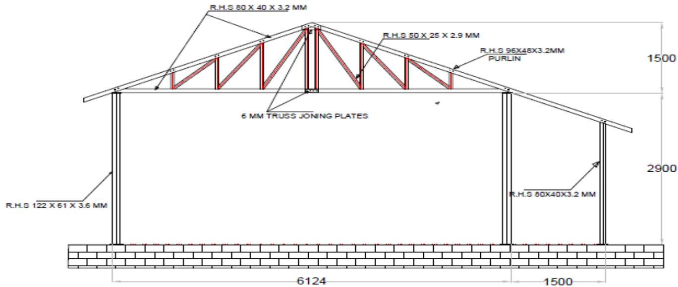
TRUSS PLAN STORE SHELTER 18.30 X 6.1 MTR
