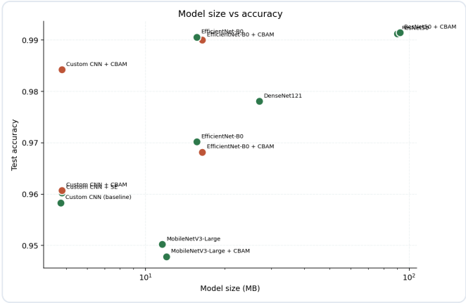
Figure 4: Pareto Frontier: Model Size (MB) vs. Test Accuracy.
