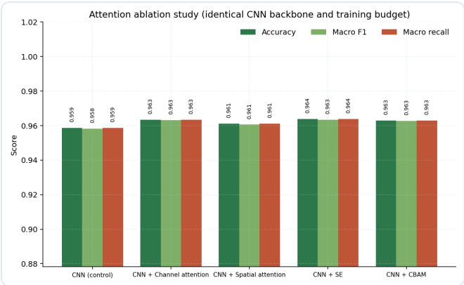
Figure 5: Ablation Arms Accuracy and Macro F1 Gains.
