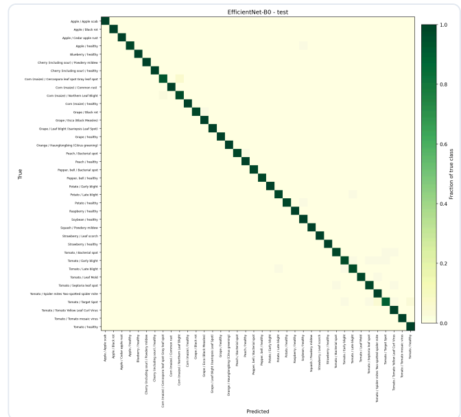
Figure 8: Normalized Test Confusion Matrix (17,572 Images).
