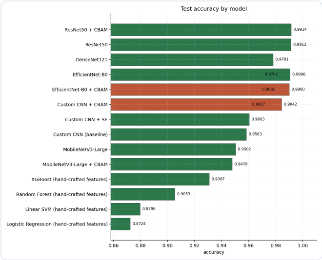
Figure 3: Test Accuracy Comparison across Model Families.
