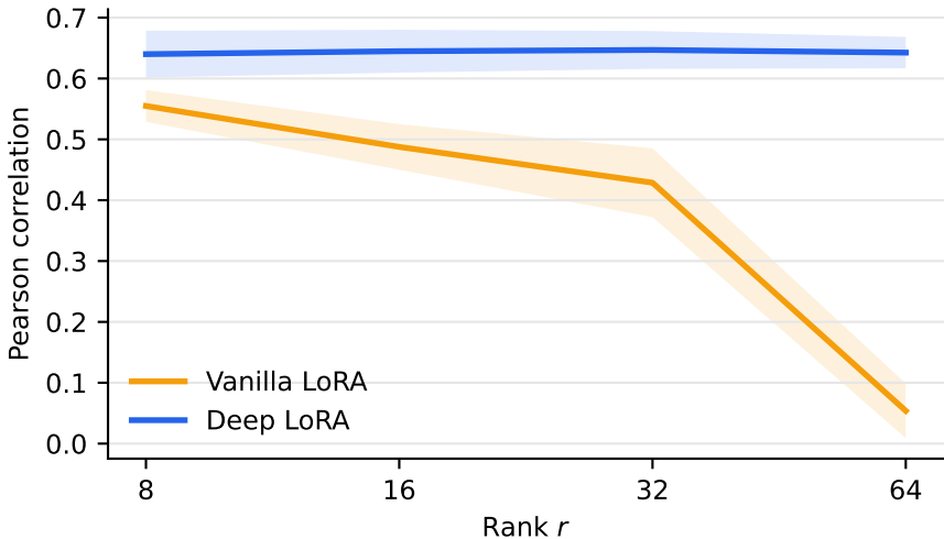
Rank robustness on STS-B
