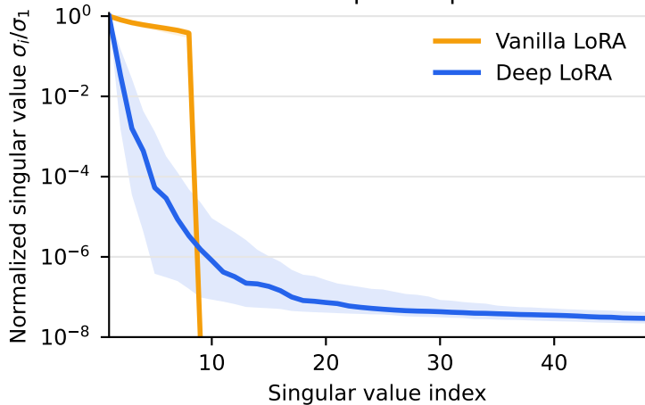
Learned update spectra
