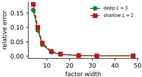
Training error
