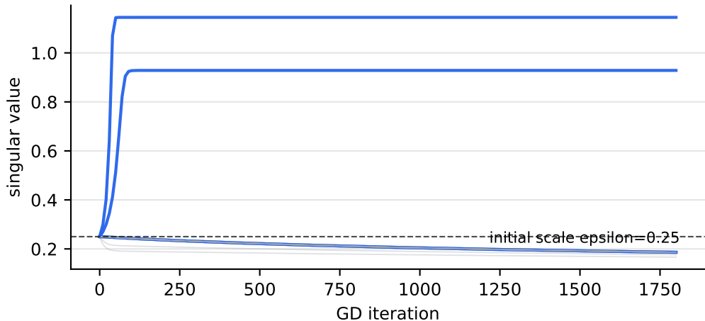
Singular values of one factor during full GD
