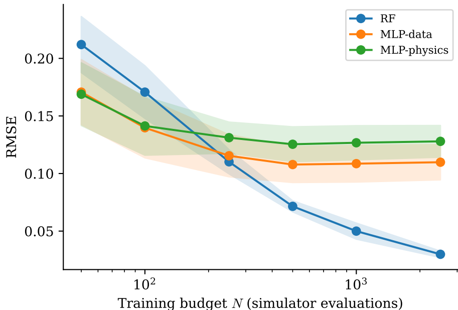
Figure A: RMSE vs. \ budget (10 seeds \times 2 strategies, shaded = std)
