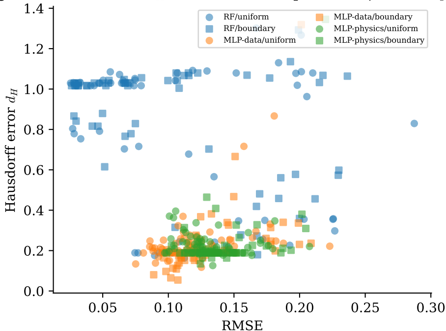
Figure C: RMSE vs. d_H , all 360 runs (Spearman \rho=-0.08 , p=0.15 )
