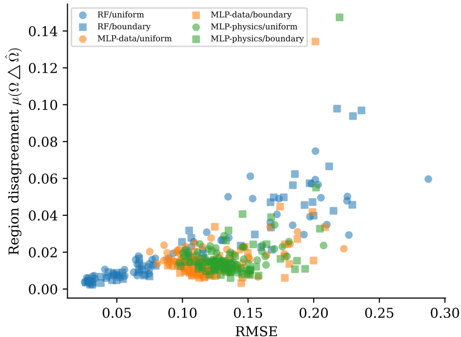
Figure D: RMSE vs. \ region disagreement, all 360 runs (Spearman \rho=0.56 , p=5.0e-31 )
